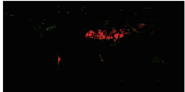
Figure 11: Emissivity category map of 1 Jan. 2001 (Upper: Red: 2, Green: 1, Blue: 0, Lower: Red: 7, Green: 4, Blue: 3)
