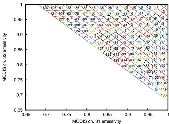
Figure 4: The emissivity category
