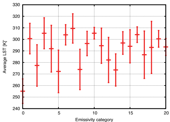
Figure 10: The average and standard deviation of LST at each category (0 – 20th. category)
