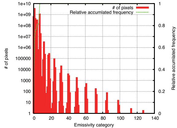
Figure 5: Total pixel of the emissivity category (All category)
