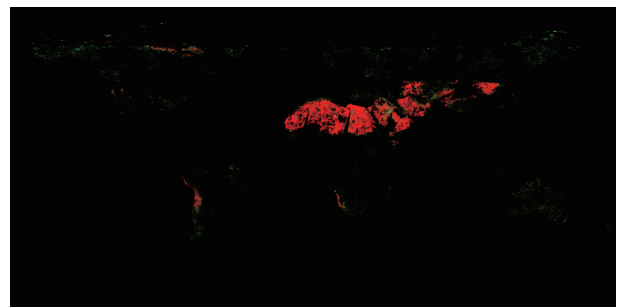
Figure 12: Emissivity category map of 1 July 2001 (Upper: Red: 2, Green: 1, Blue: 0, Lower: Red: 7, Green: 4, Blue: 3)
