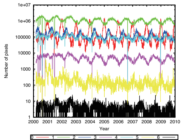
Figure 7: Daily variation of the pixel number of the emissivity category (0–6th. category)
