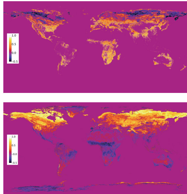
Figure 14: Correlation coefficient between a and NDVI (Upper), NDWI (Lower)
