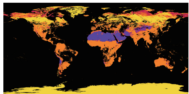
Figure 1: MODIS ch. 31 emissivity on 1 Jan. 2001
