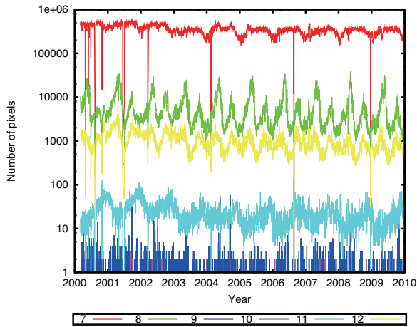
Figure 8: Daily variation of the pixel number of the emissivity category (7–12th. category)
