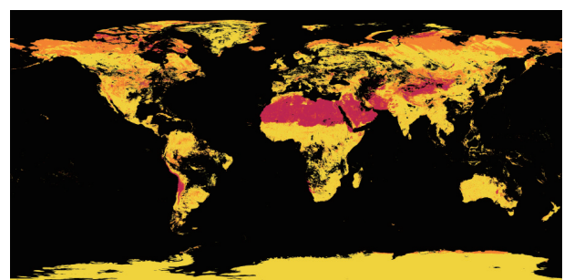
Figure 2: MODIS ch. 32 emissivity on 1 Jan. 2001
