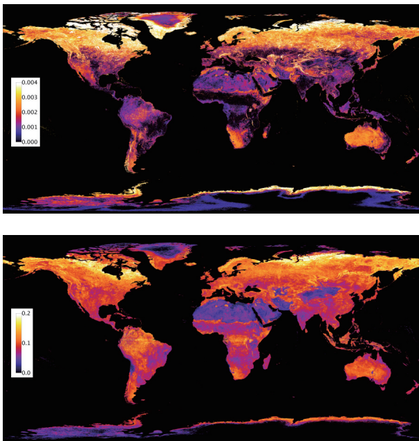
Figure 13: Standard deviation of \bar{\varepsilon} (Upper) and a (Lower)
