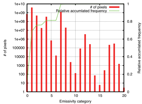
Figure 6: Total pixel of the emissivity category (0–20th. category)
