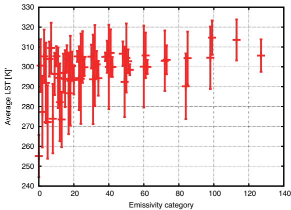
Figure 9: The average and standard deviation of LST at each category (All category)
