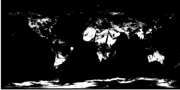
Figure 3: The mask image on 1 Jan. 2001
