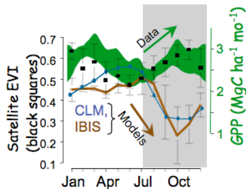
Figure 1. Contrasting model, flux tower, and satellite data forest responses to seasonal drought periods.
