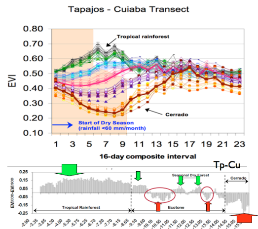
Figure 2. Varying tropical forest responses to seasonal drought along a transect from northern to southern Amazon forests and the cerrado region.
