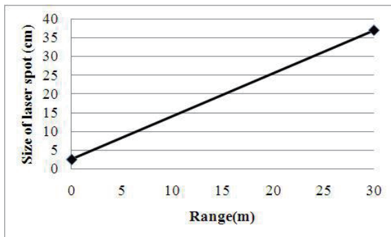
Figure3. Relation between range and size of laser spot of the SICK Laser Measurement Sensor (LMS) 200
