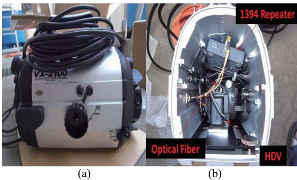
Figure 8. (a) The waterproof case, (b) HDV, 1394 repeater and optical fiber
