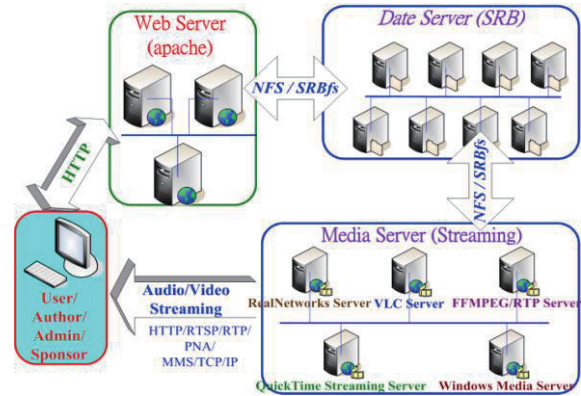
Figure 5. Illustration of the schematic view of stream servers, and storage pool
