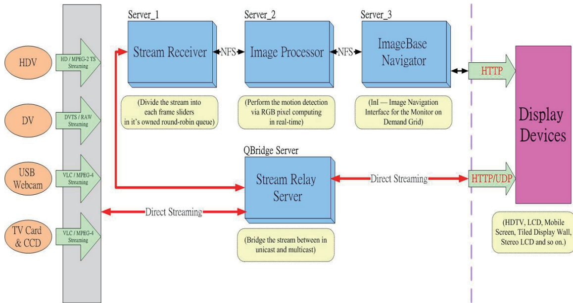
Figure 1. Architecture blocks and stream pipeline
