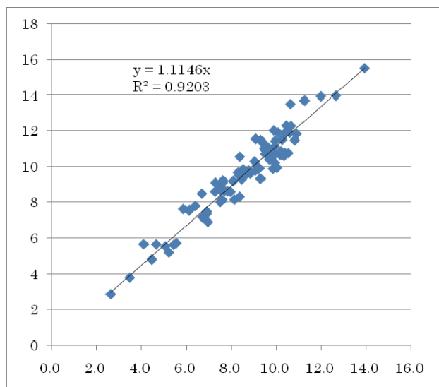
Figure 5. Comparison of NPP between Satellite and ground (tC)
