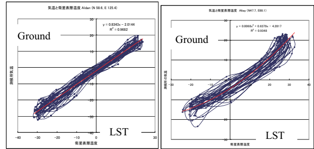
Figure 3. Relations between LST and ground temperature
