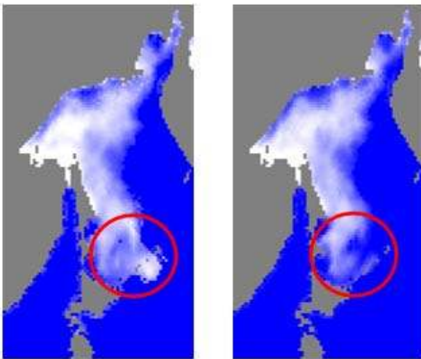
(a) 15% rejection (b) Three days minimum Figure 7. Comparison of false sea ice reduction effect (Sea of Okhotsk, SSM/I April 5, 2000)
