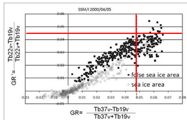
Figure 5. Scatter plot of GR(37/19) and GR(22/19) (Sea of Okhotsk, SSM/I April 5, 2000)
