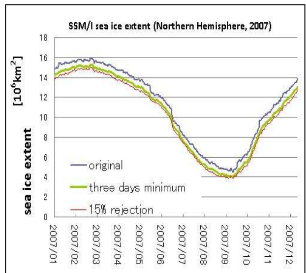
(b) Sea ice extent of Northern Hemisphere (2007)
