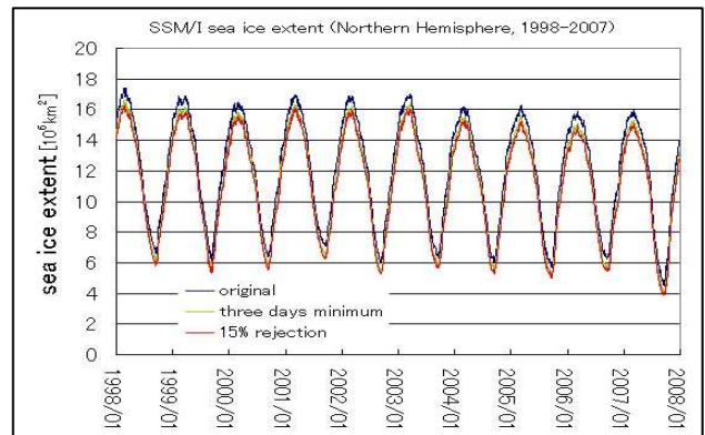
(a) Sea ice extent of Northern Hemisphere (1998-2007)
