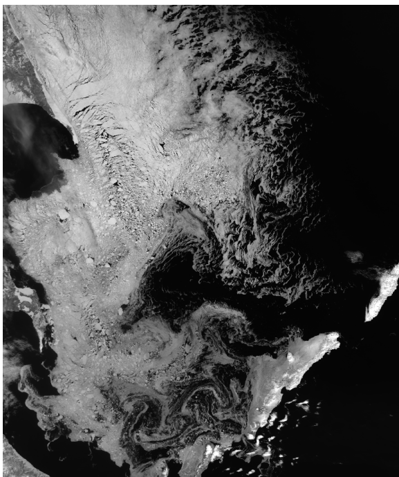
Figure 3. MODIS image of the Sea of Okhotsk for April 4, 2000.
