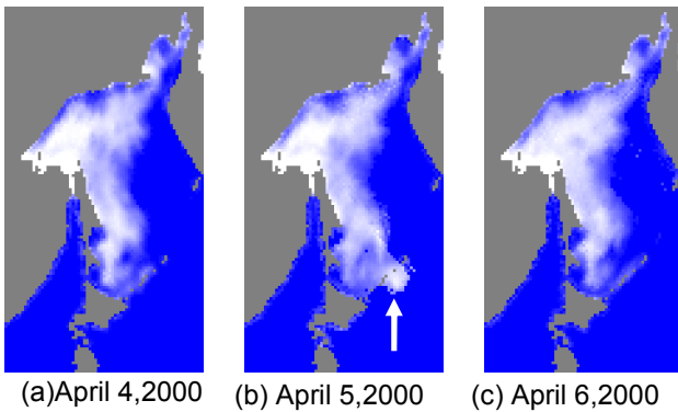
Figure 2. SSM/I sea ice concentration images of the Sea of Okhotsk
