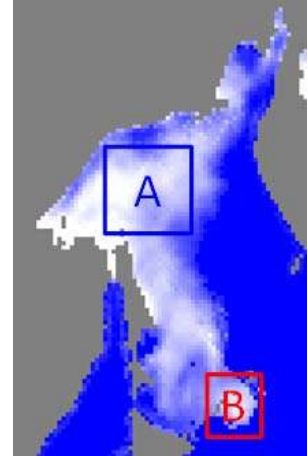
Figure 4. Extraction of sea ice area(A) and false sea ice area(B) in the SSM/I sea ice concentration image of the Sea of Okhotsk. (April 5, 2000)
