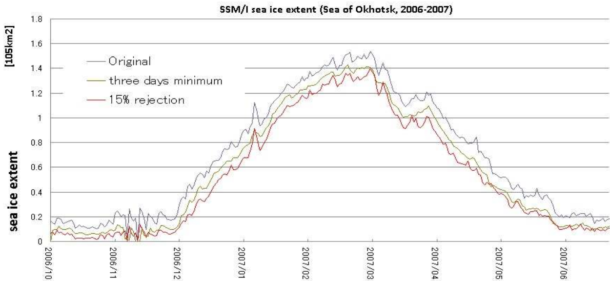
Figure 9. Comparison of the sea ice extent difference between each method for the Sea of Okhotsk (2006-2007).
